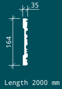
Moulding 1.51.501
