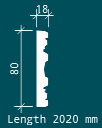
Moulding 1.51.504
