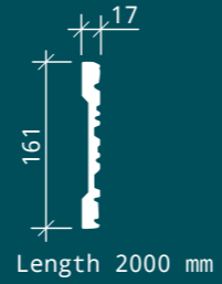
Moulding 1.51.510
